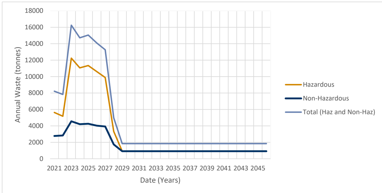
Figure 5-3: Projected Waste Volumes 2021–2046 Total Waste by Type Offshore Generation/Onshore Management Approved & Theoretical Projects
