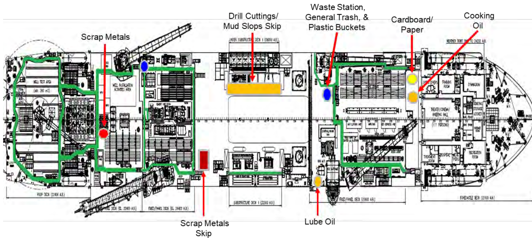
Figure 4-11: Example Noble Drill Ship Waste Storage Locations
