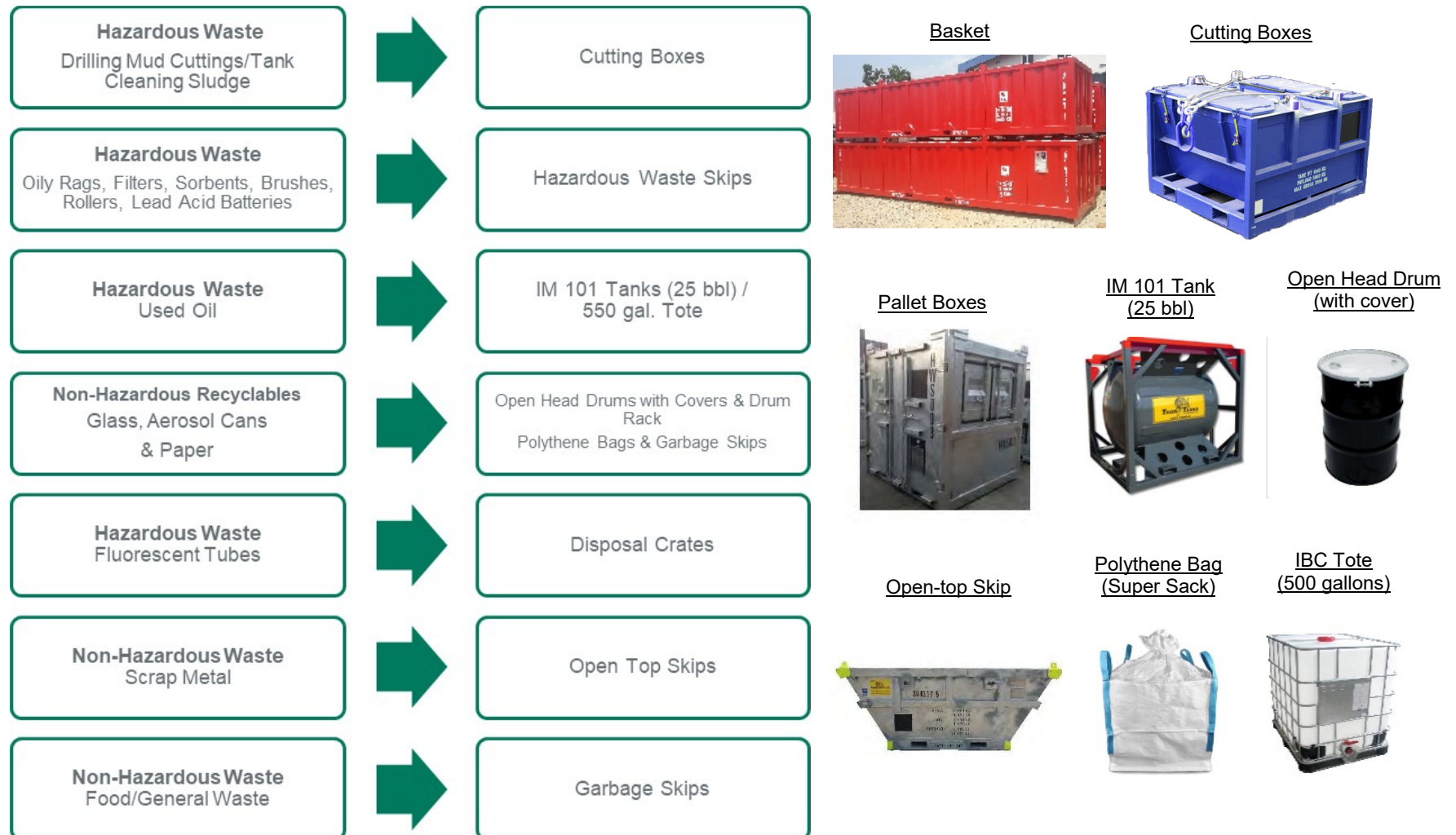
Figure 6-4: Waste Storage and Transport Containers
