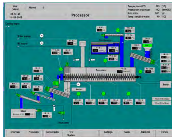
Typical HTDU Control Screen
