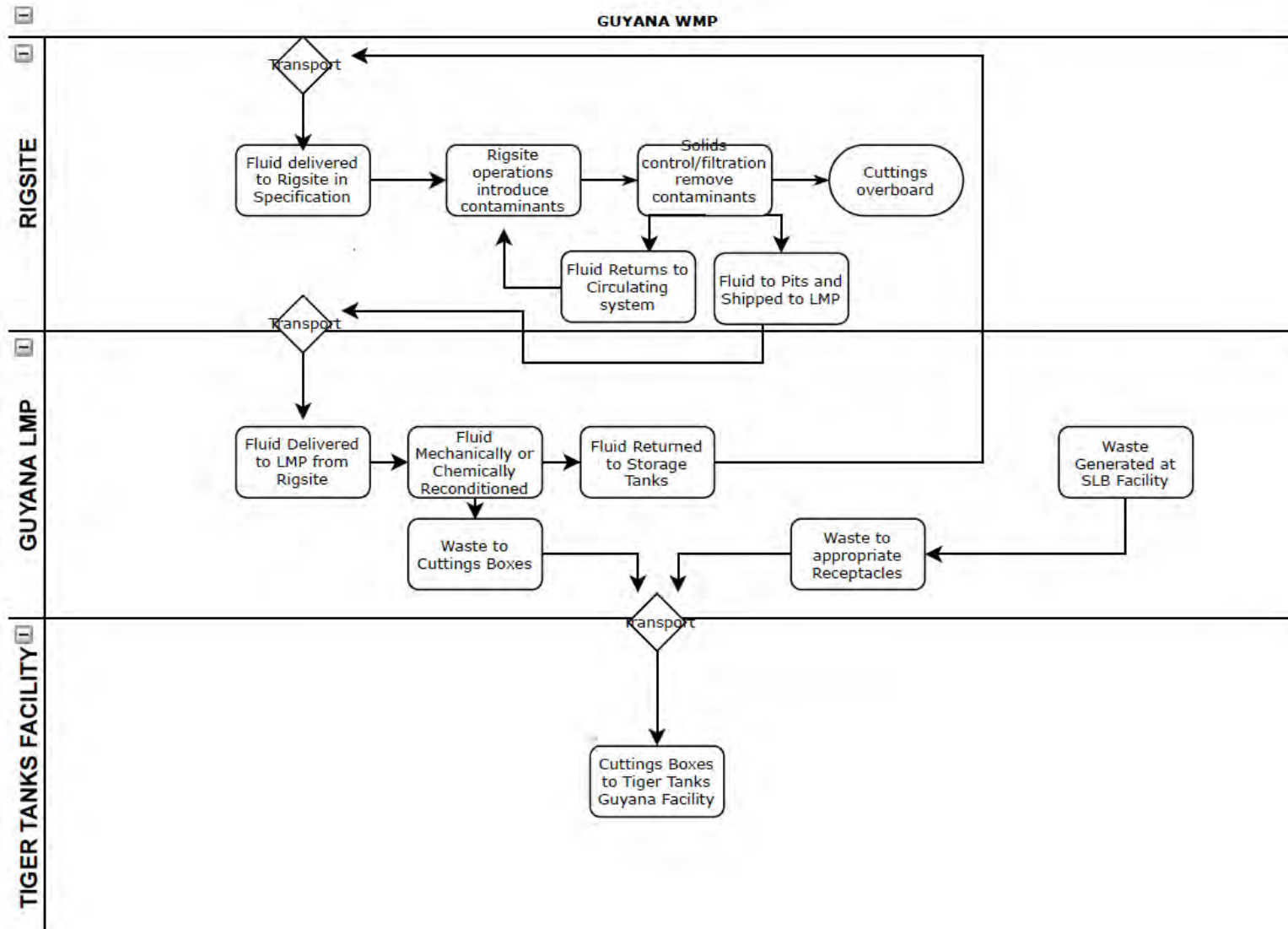
Figure 4-57: Example Liquid Mud Plant Workflow Diagram
