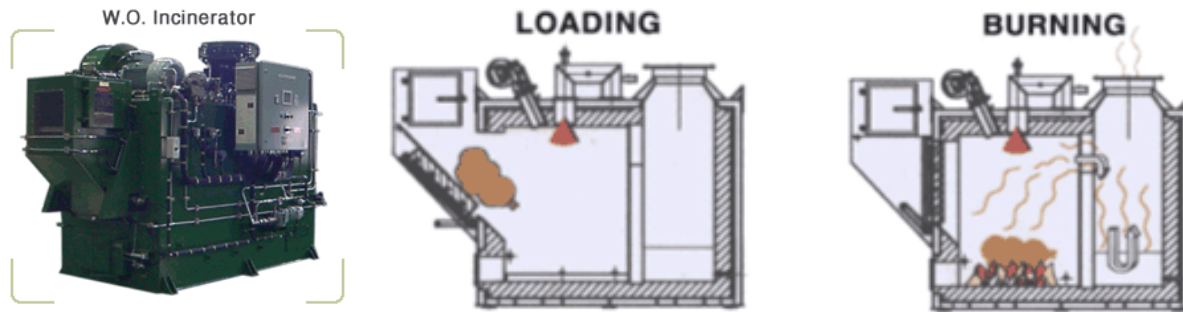
Figure 4-26: Incineration
