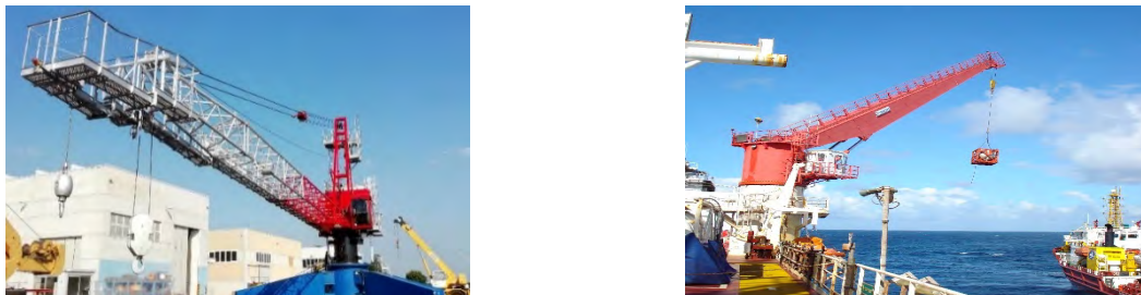
Figure 4-15: Drill Ship/FPSO Transfer of Support Vessel Example
