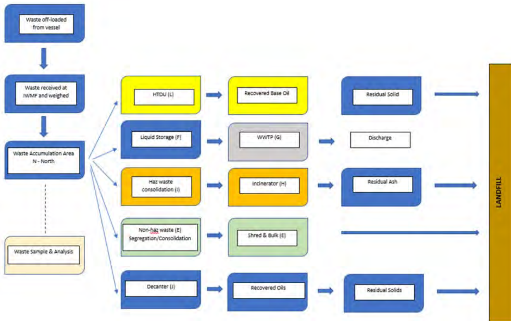
Figure 4-49: SES IWMF Operations Flow Diagram
