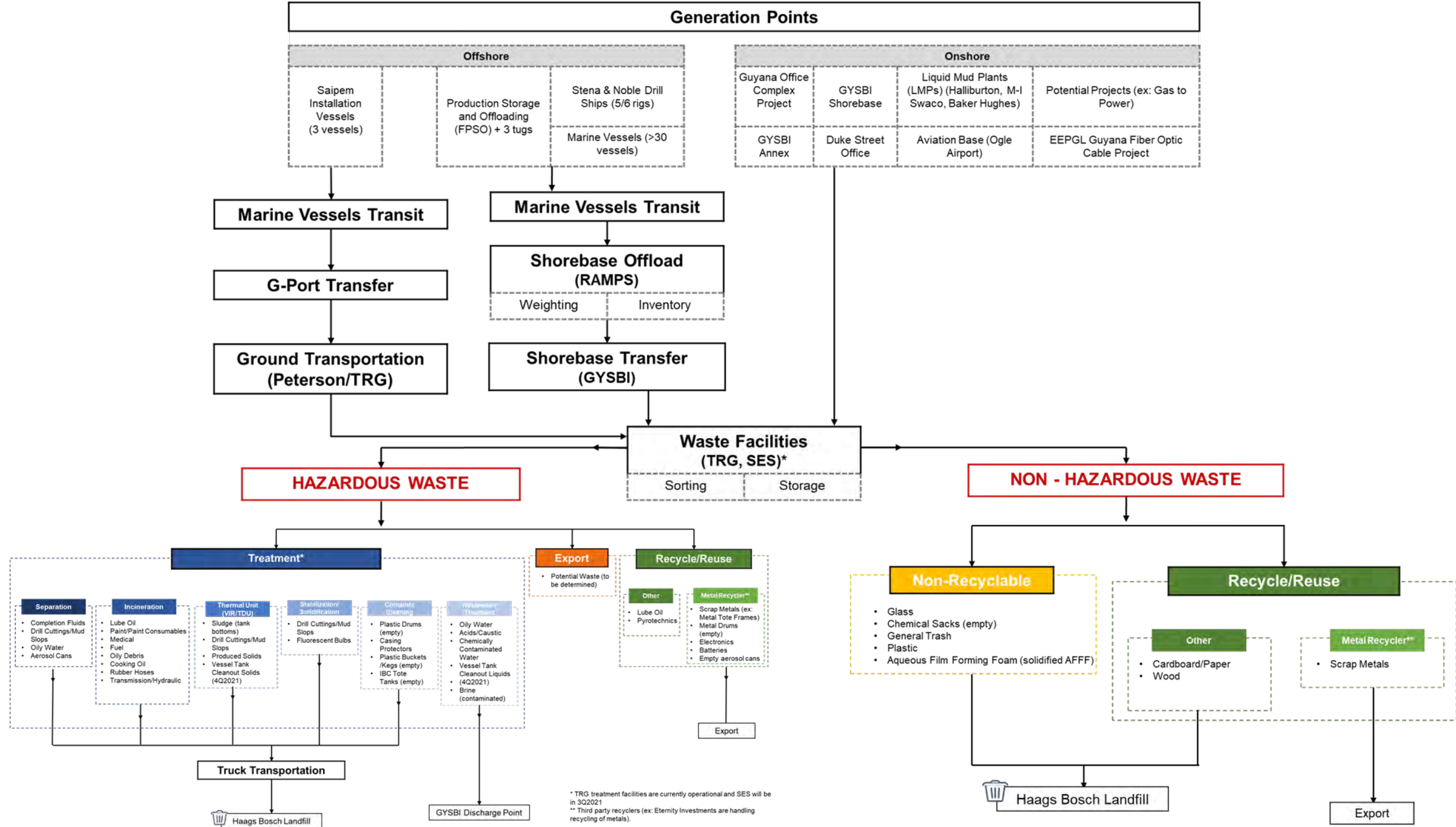
Figure 4-3: Generation Point Flow Diagram
