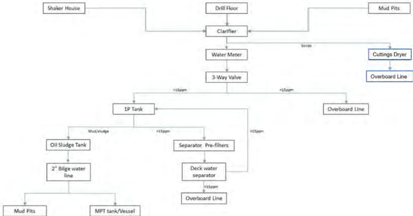
Figure 4-21: Noble Drill Ships Drilling Wastes Management
