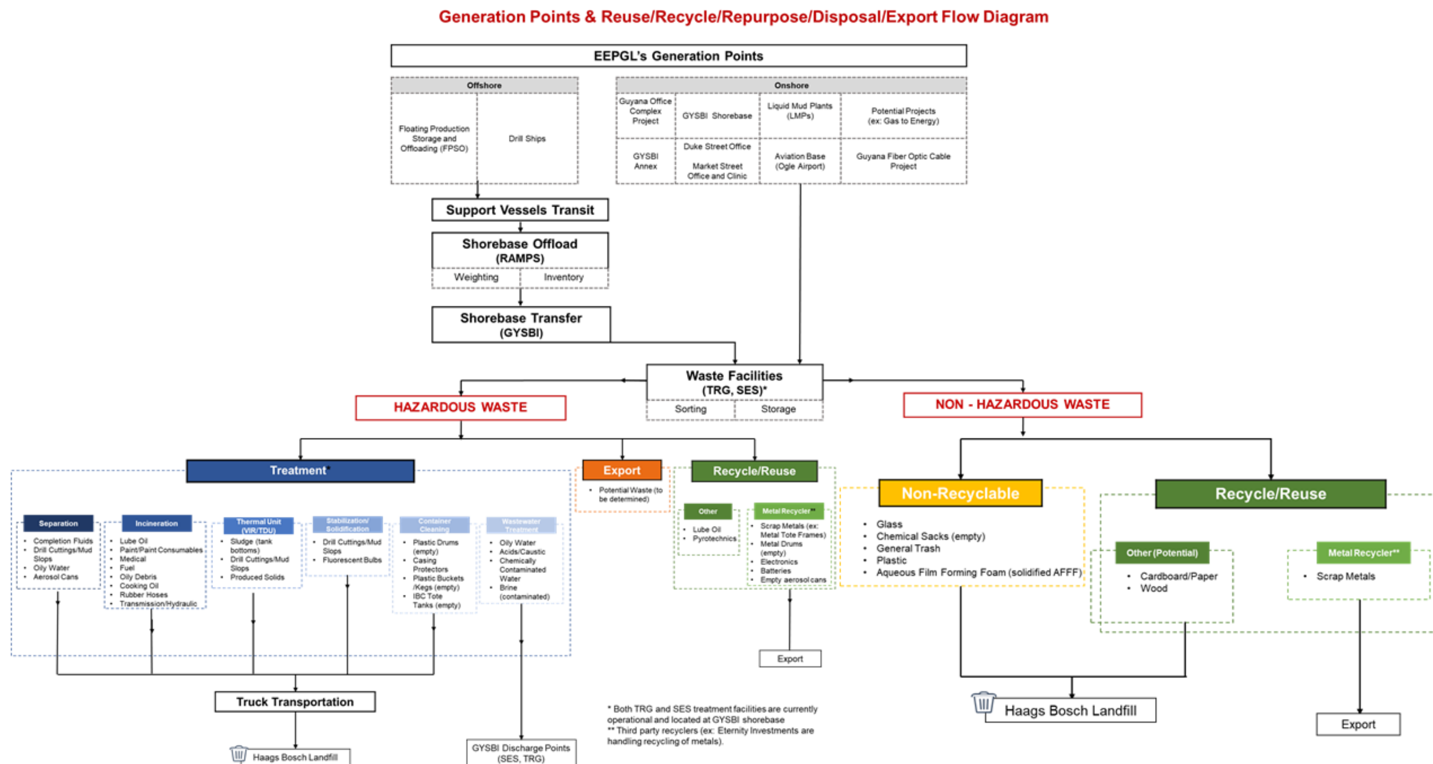
Figure 6-3: EEPGL Generation Points Flow Diagram
