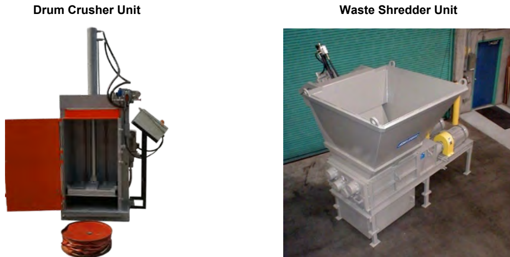
Figure 4-56: Solids Reduction Measures
