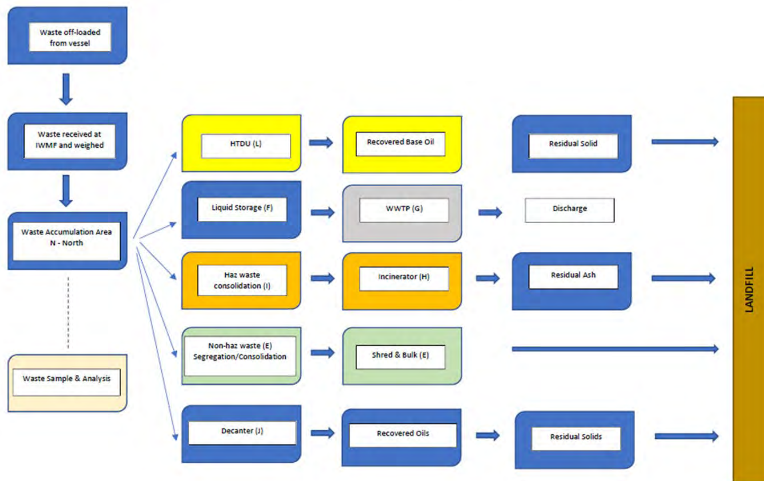
SES Integrated Waste Management Facility Flow Diagram (1)
