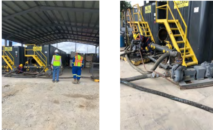
Figure 4-44: Frac Tank Storage
