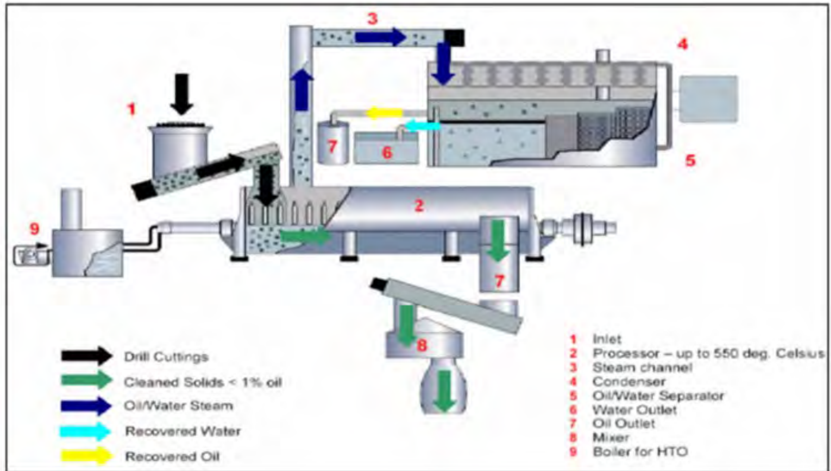
Figure 4-50: Thermal Desorption Treatment
