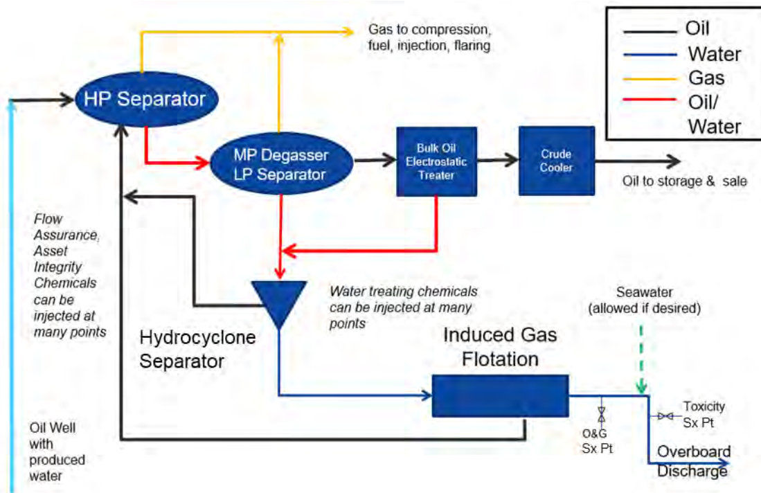
Figure 4-27: Typical Produced Water Source and Treatment
