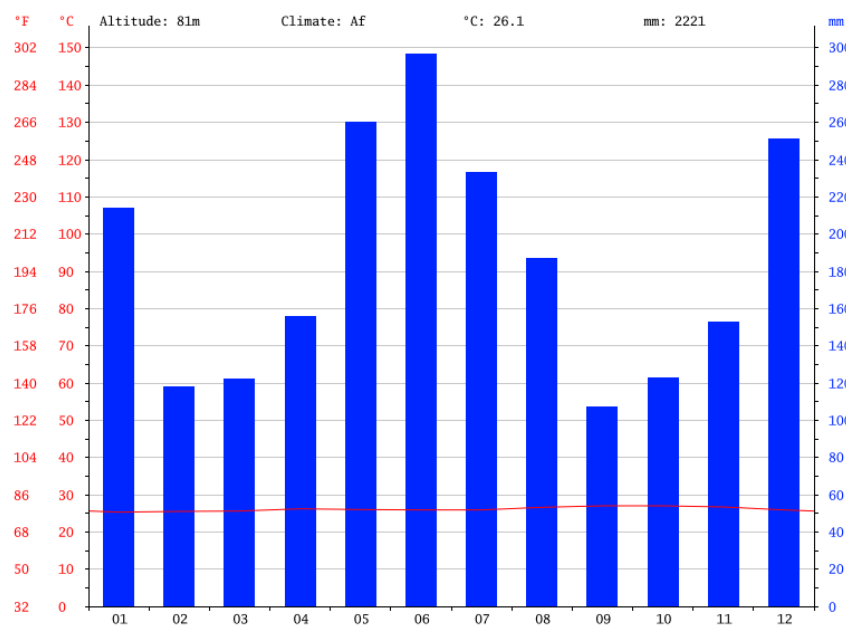
Figure 22: Climograph for Aranka, left bank Cuyuni River, Region 7.
