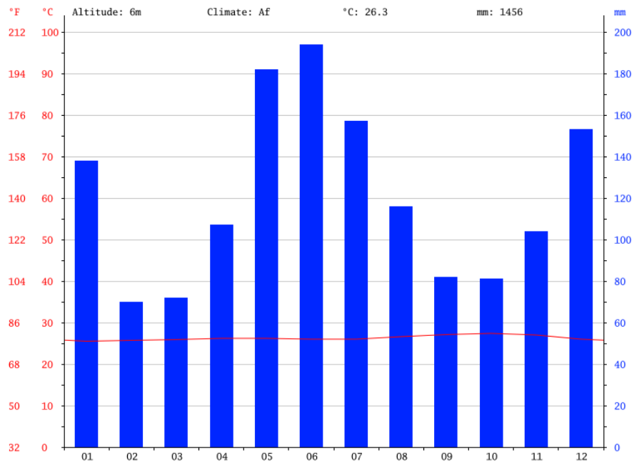
Figure 21: Climograph 12 for Iteballi, left bank Mazaruni River 13 , Region 7
