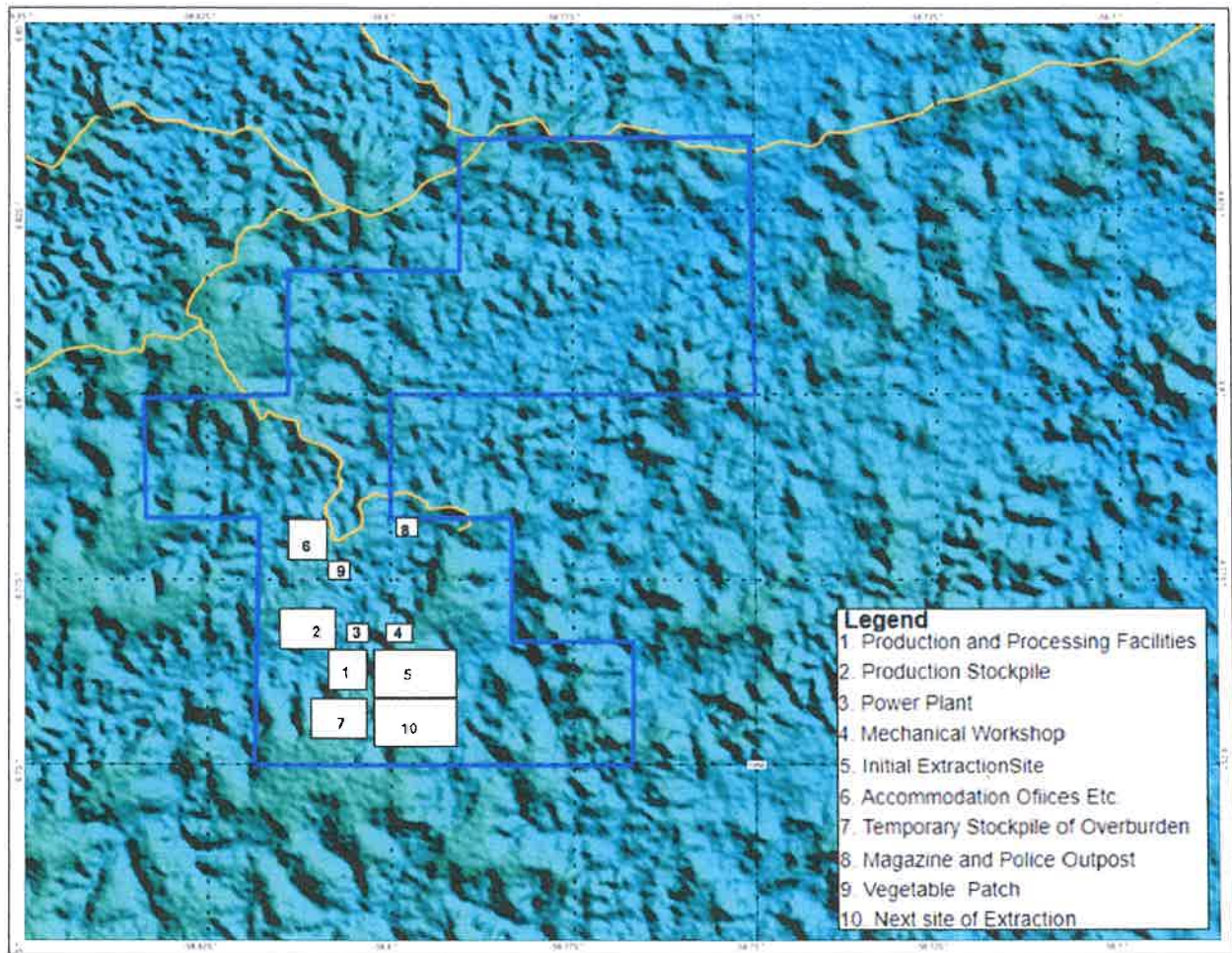
Map 3.2: Proposed Layout and Site plan for the quarry development.
