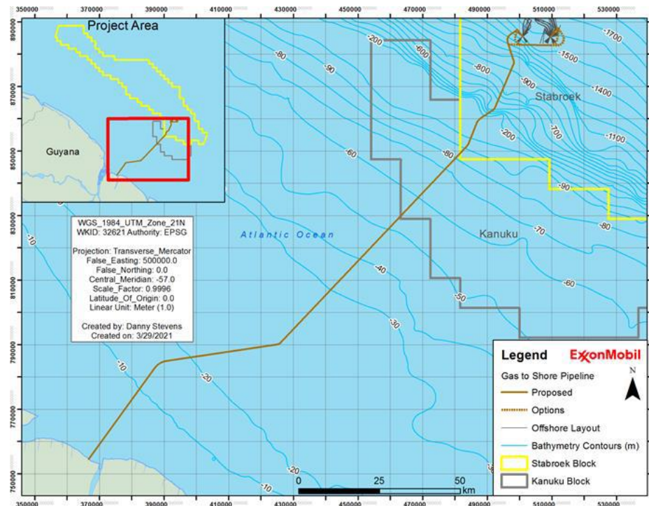
Figure 1 Project Schematic
