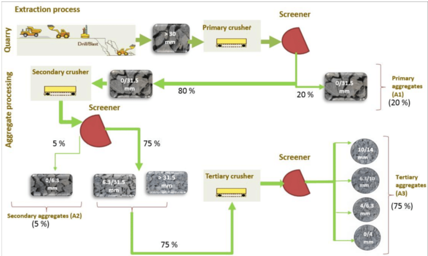
CONCEPTUAL MINING PROCESS
