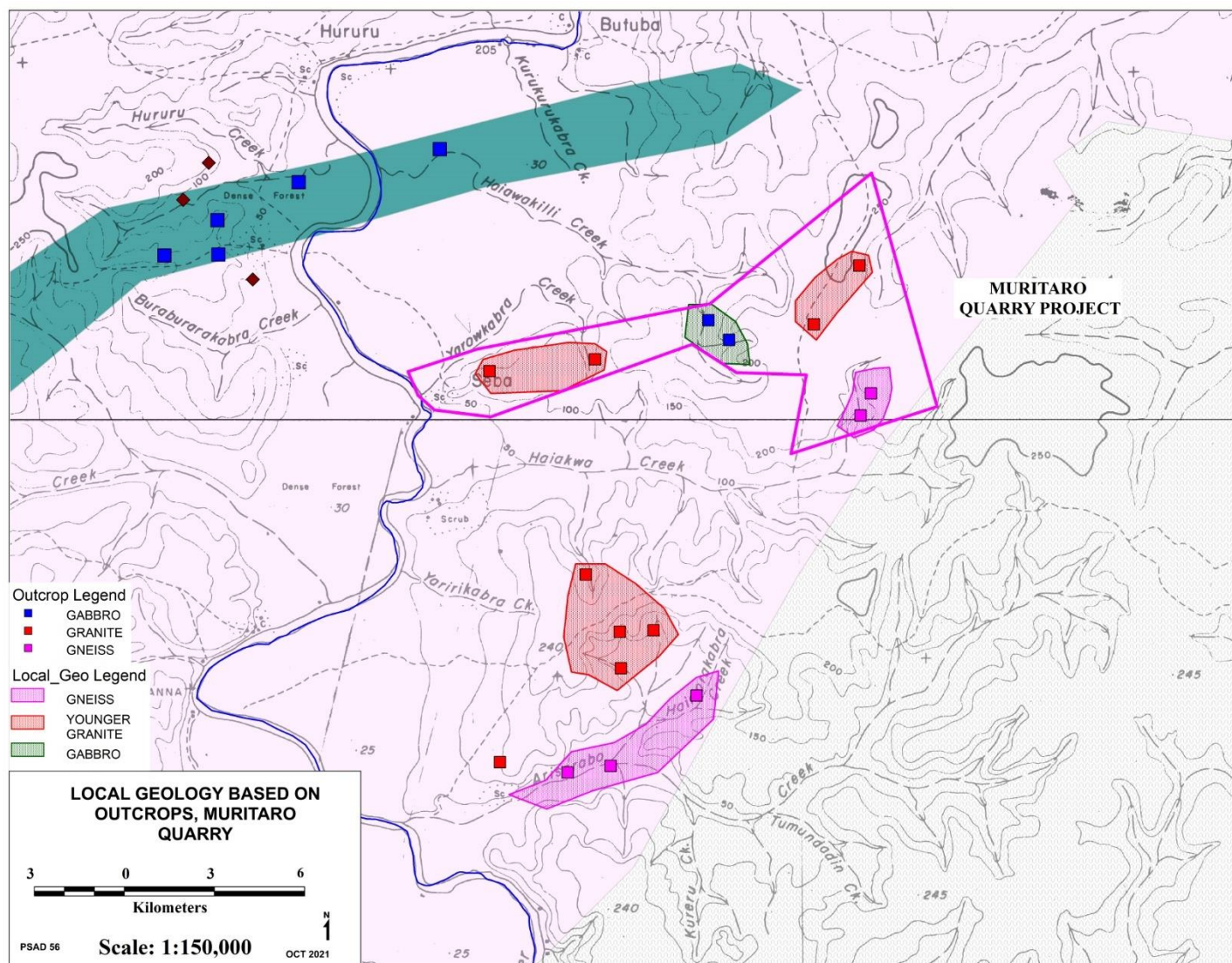
Figure 5: Local Geology Map for “MVCNTR” Muritaro Quarry Project based on Field Mapping
