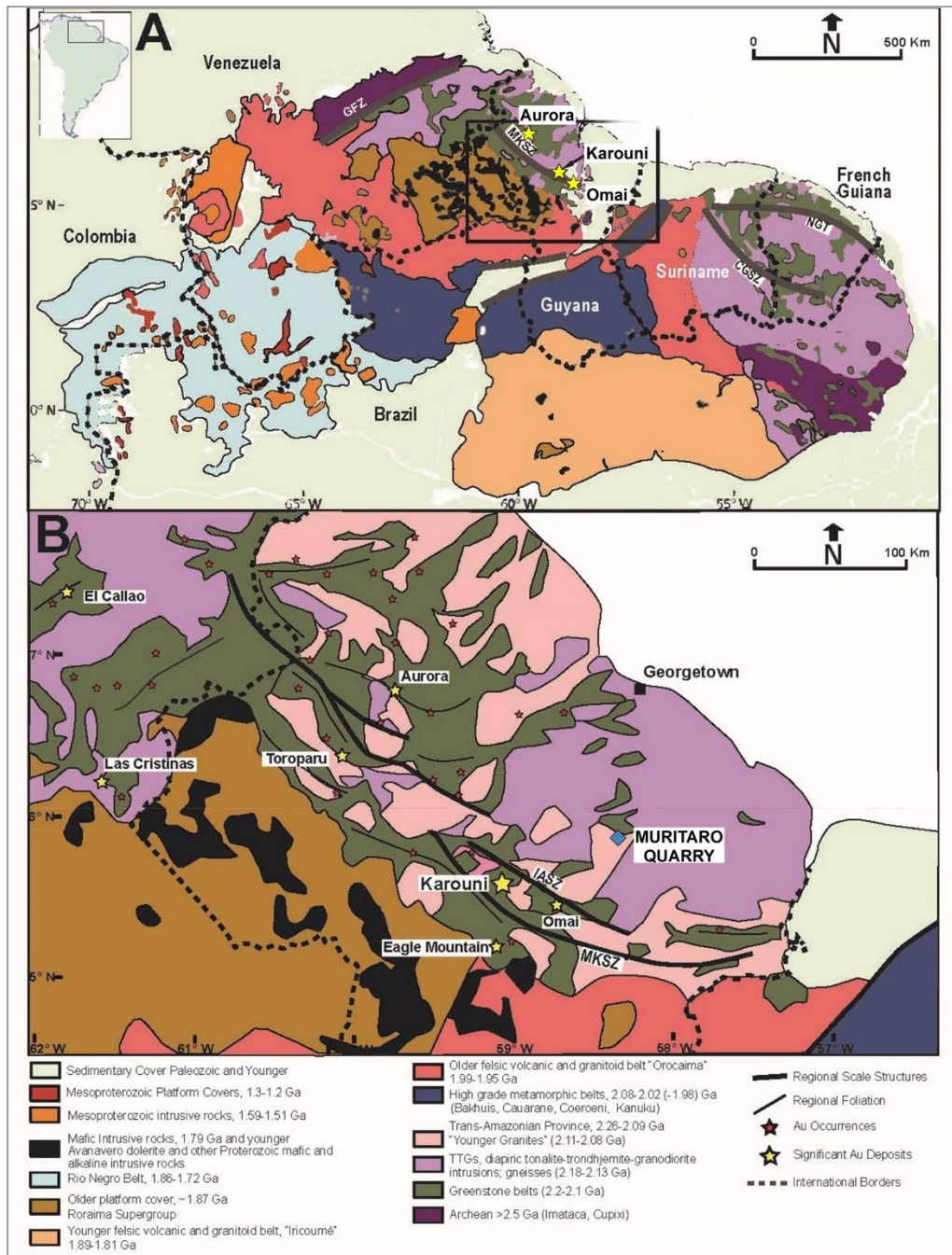
Figure 3: Regional Geology and Deposits, Guyana 5
