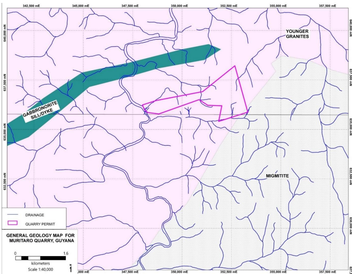
Figure 4: Regionally Geology map for Muritaro area, "MVCNTR" Quarry Project
