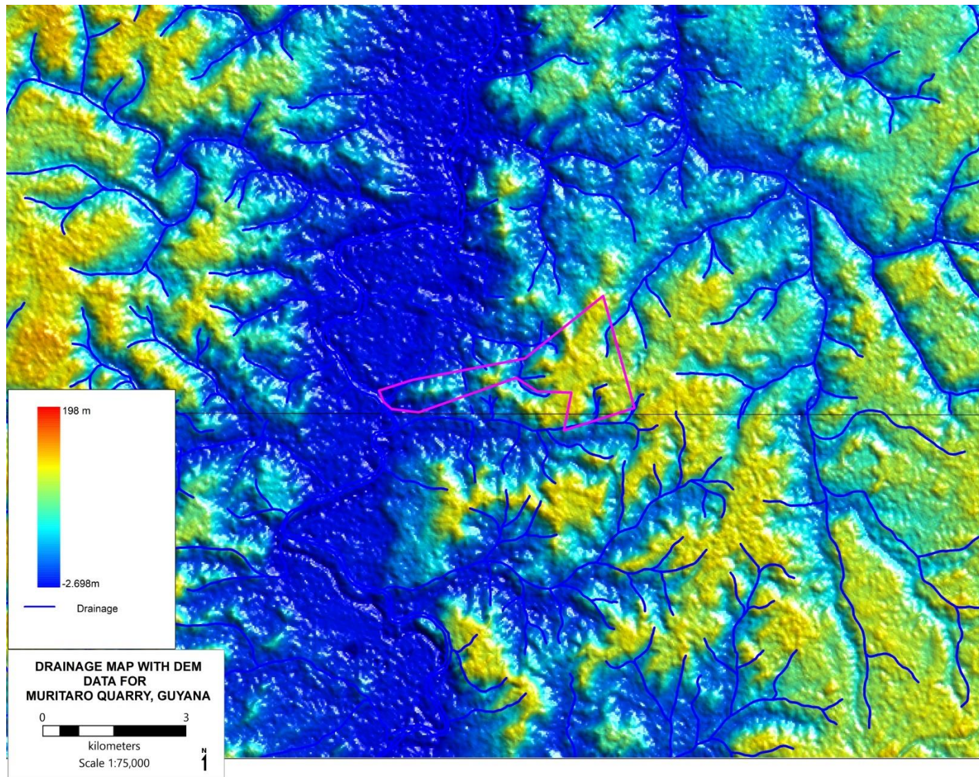
Figure 8: Drainage map for “MVCNTR” Muritaro Quarry Project based on Field Traverse and DEM (elevation) regional data
