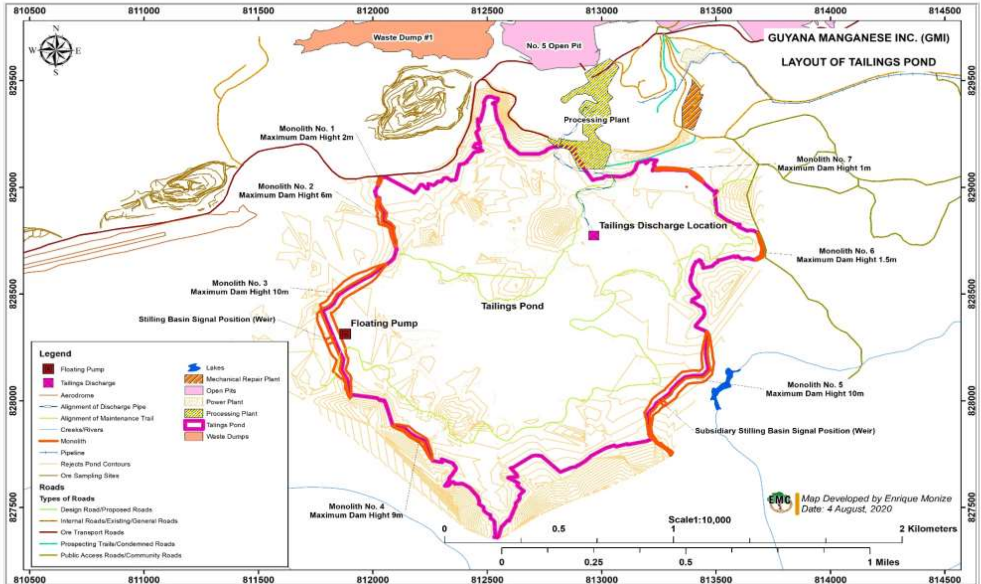
Figure 16-7: Tailings Rejects Pond
