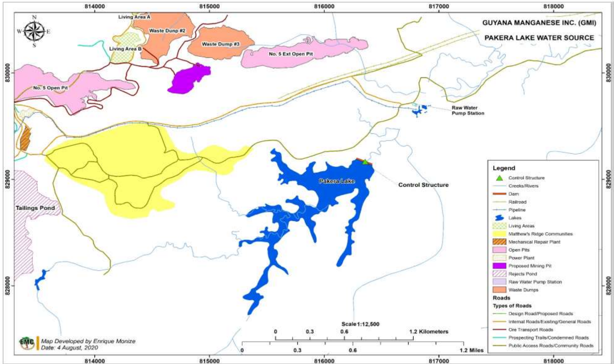
Figure 4-9: Pakera Lake and Water Supply Components
