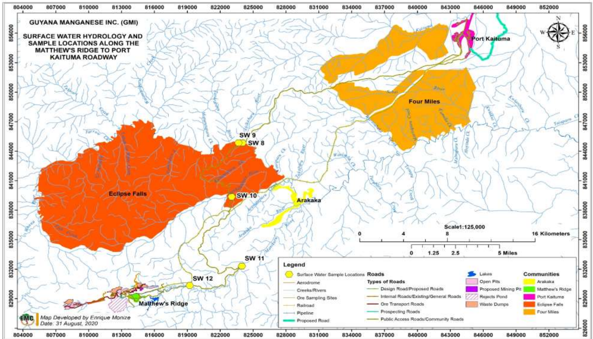
Figure 8-17: Surface Water Hydrology and Sample Locations along the Matthew's Ridge to Port Kaituma Roadway
