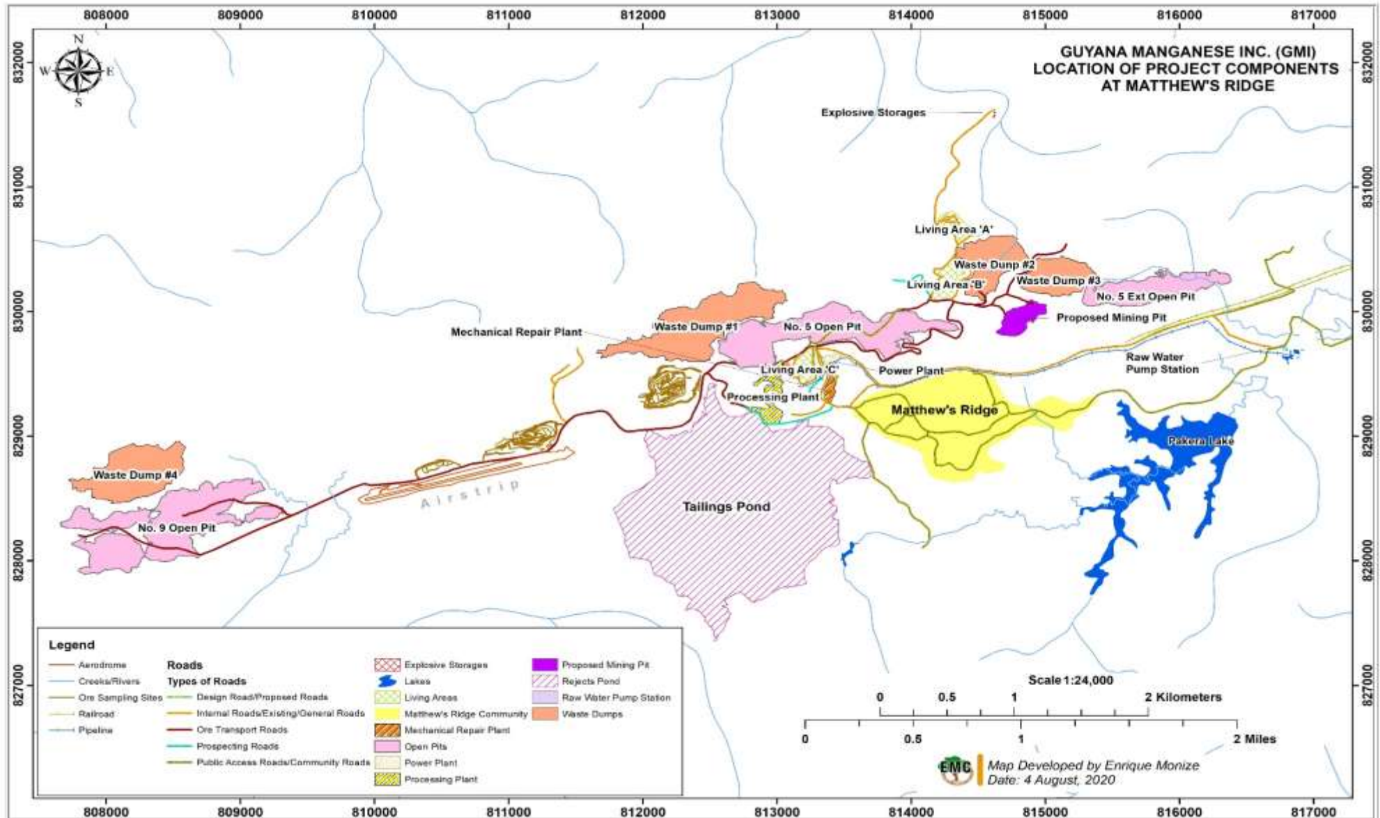
Figure 4-3: Location of Project Components at Matthew's Ridge
