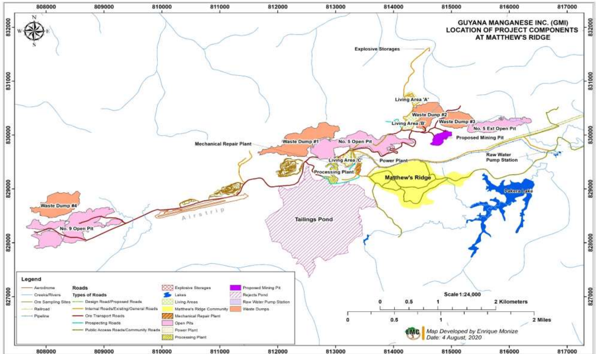
Figure 17-13: Facilities Layout at Matthew's Ridge
