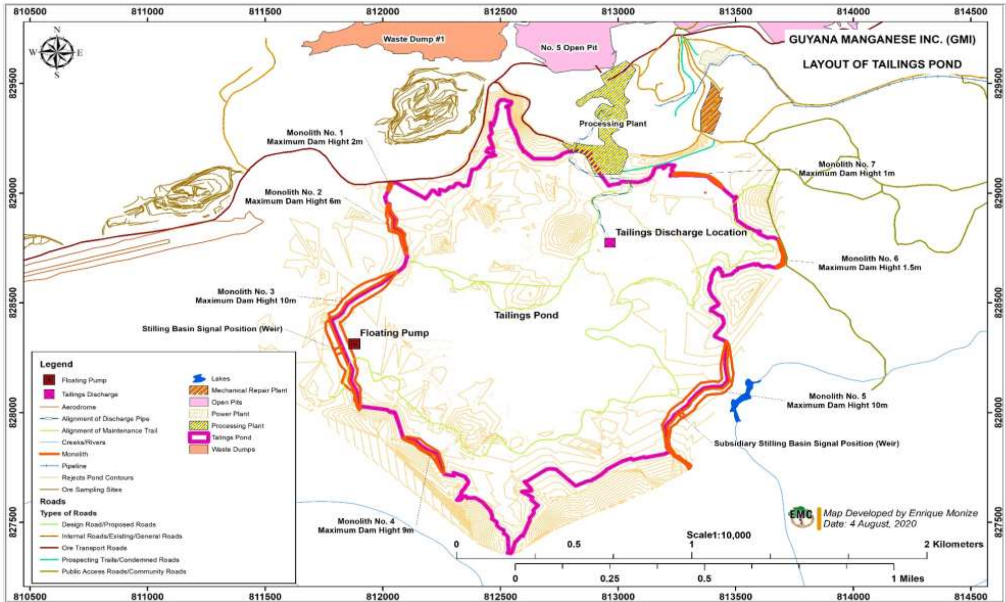
Figure 4-8: Layout of the Tailings Pond
