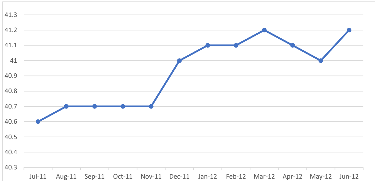
Figure 10-1: PM 10 Concentration (µg/m³) in the Measurements Conducted Over the Period July 2011 to June 2012
