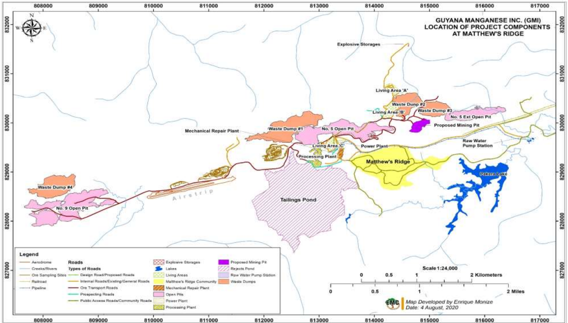
Figure 16-8: Layout of Project Facilities Showing the Relative Positions of the Waste Dumps and Rejects Ponds to other Project Components
