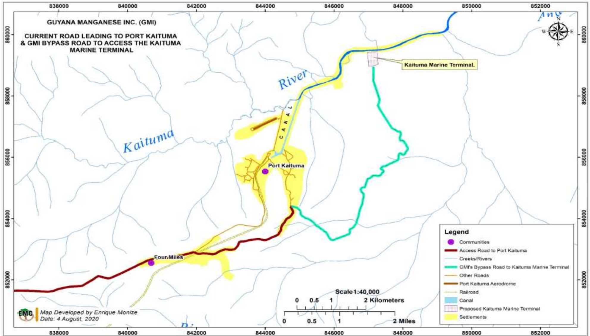
Figure 5-2: Public Roads Leading to Port Kaituma and Bypass Road Constructed by GMI
