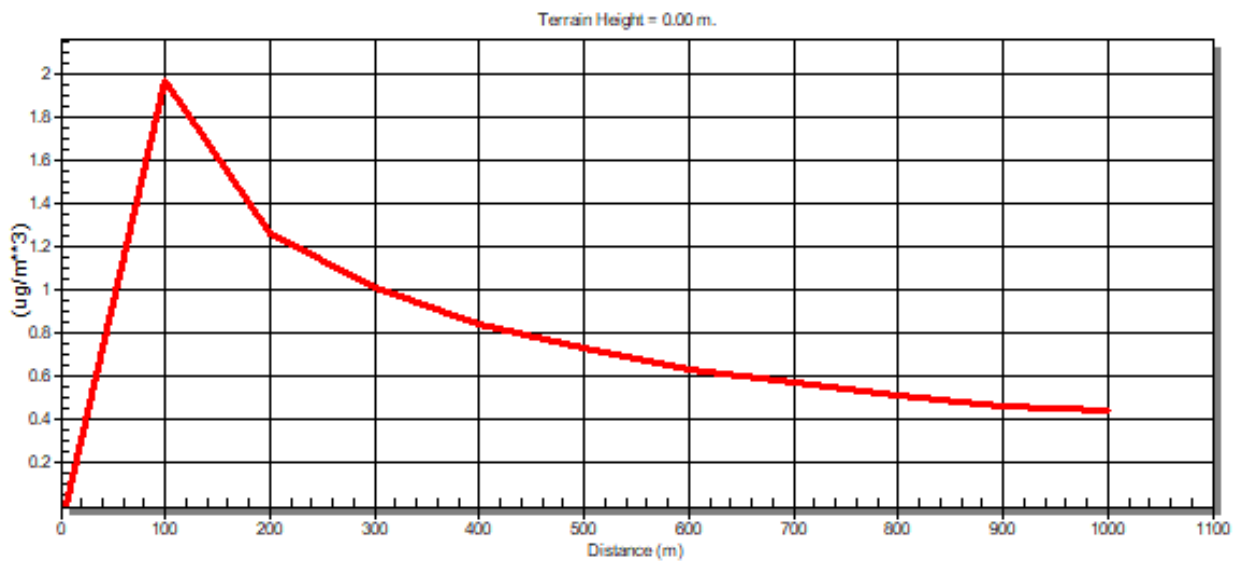
Figure 10-8: Dispersion Model for PM 10 for the Matthew's Ridge Power Plant
