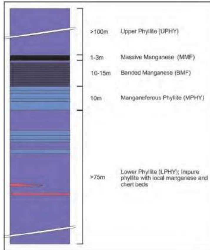
Figure 9-8: Schematic Stratigraphic Column of the MRF
