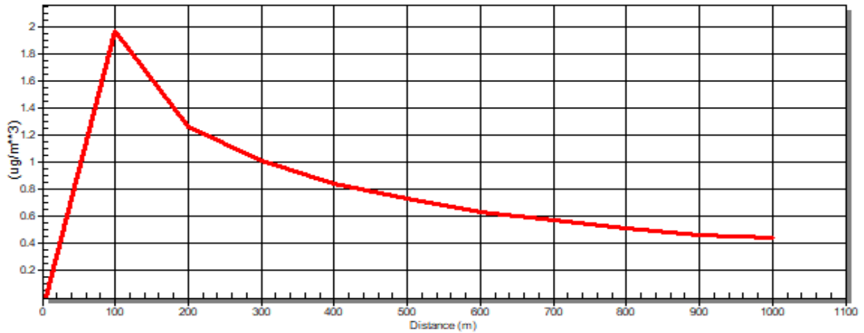
Figure 10-5: Dispersion Model for Nitrous Oxides (NOx) for the Matthew's Ridge Power Plant
