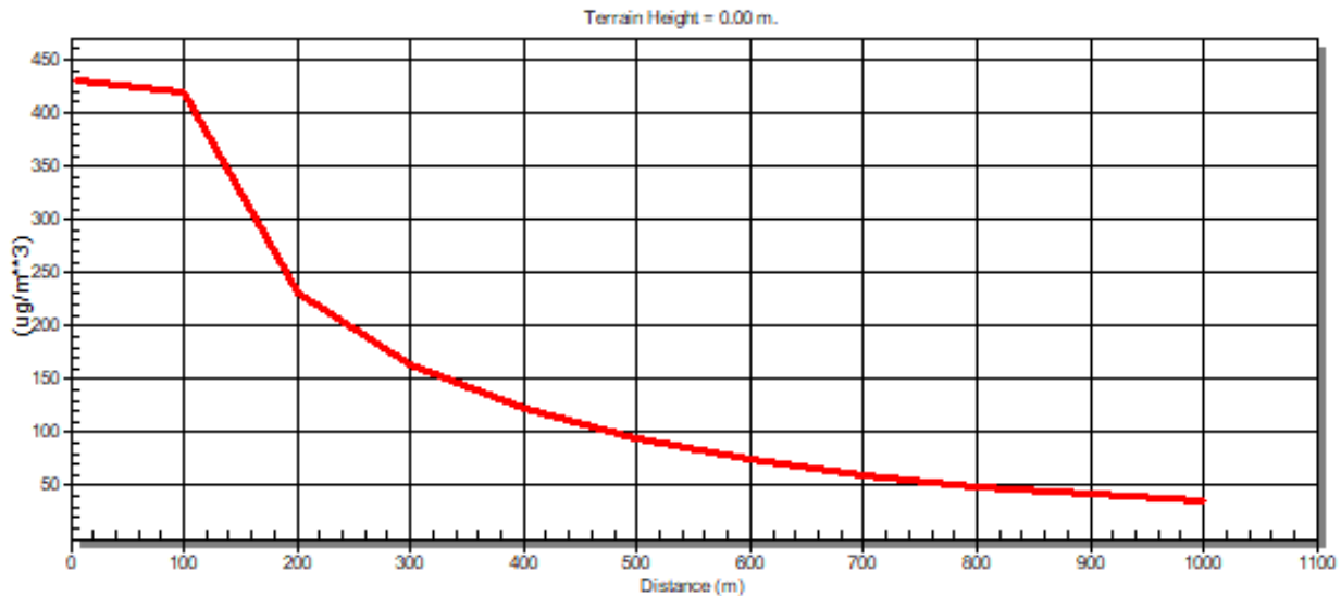
Figure 10-4: Dispersion Model for Total Suspended Particulates (TSP)
