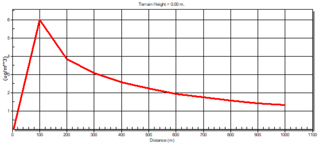
Figure 10-6: Dispersion Model for Carbon Monoxide (CO) for the Matthew's Ridge Power Plant
