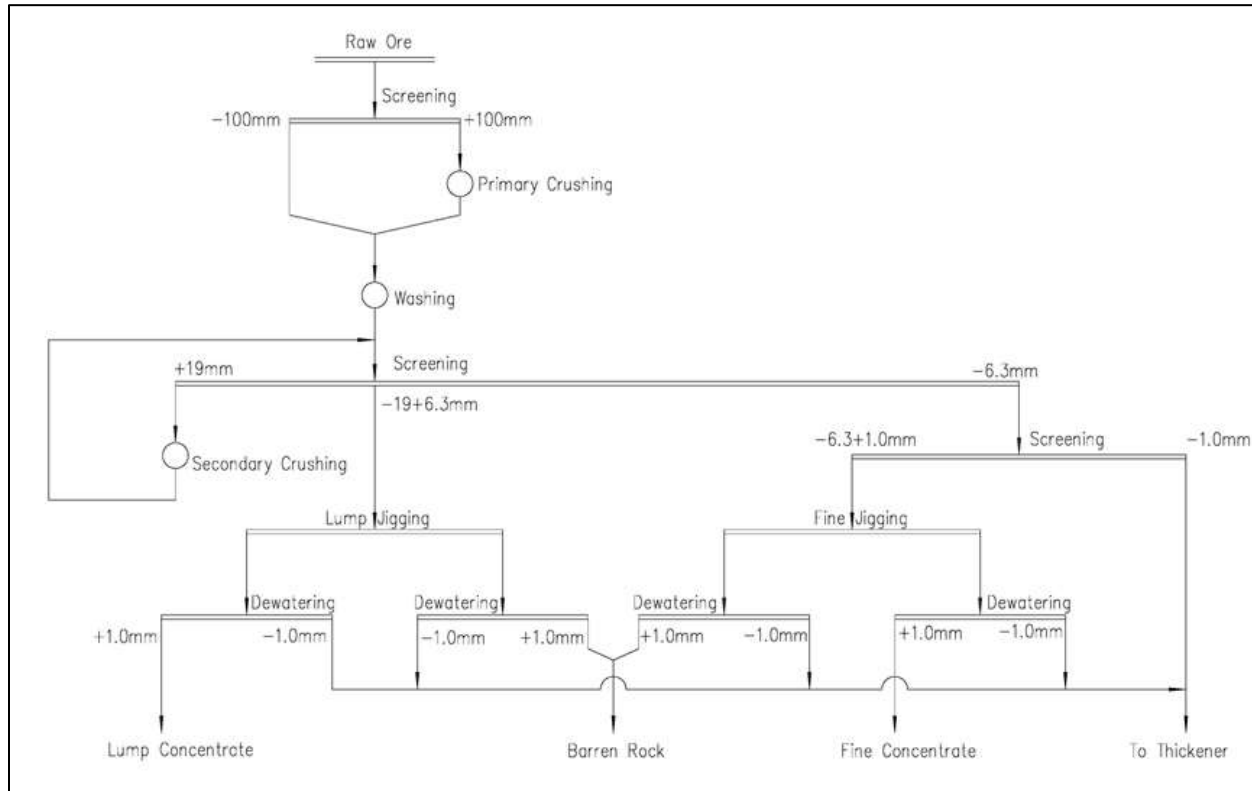
Figure 4-11: Process Flow Sheet
