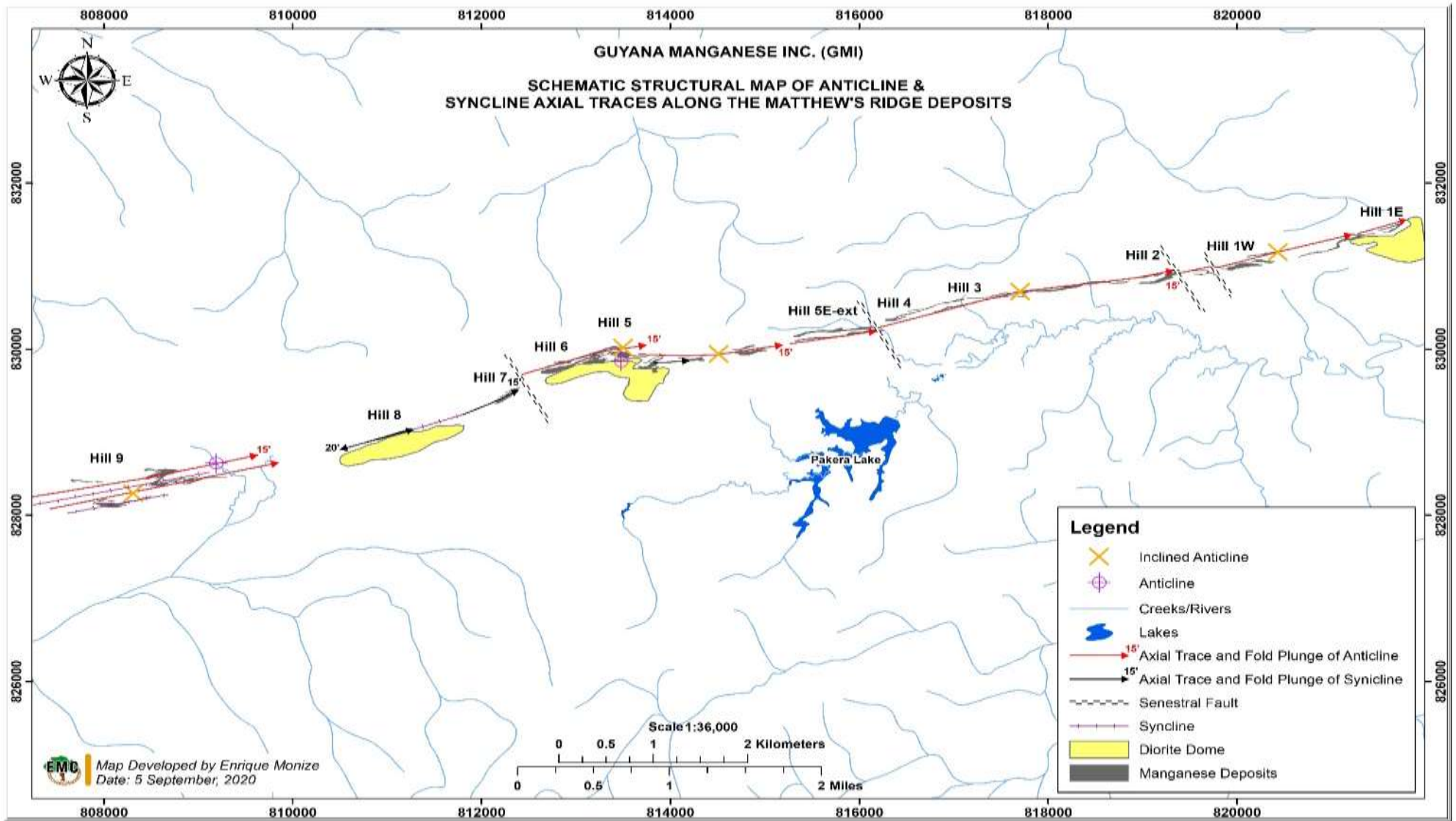
Figure 9-12: Schematic Structural Map of Anticline and Syncline Axial Traces along the Matthews Ridge Deposits
