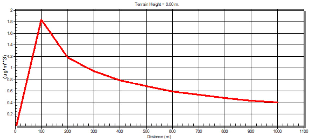
Figure 10-7: Dispersion Model for Sulphur Oxides (SOx) for the Matthew's Ridge Power Plant
