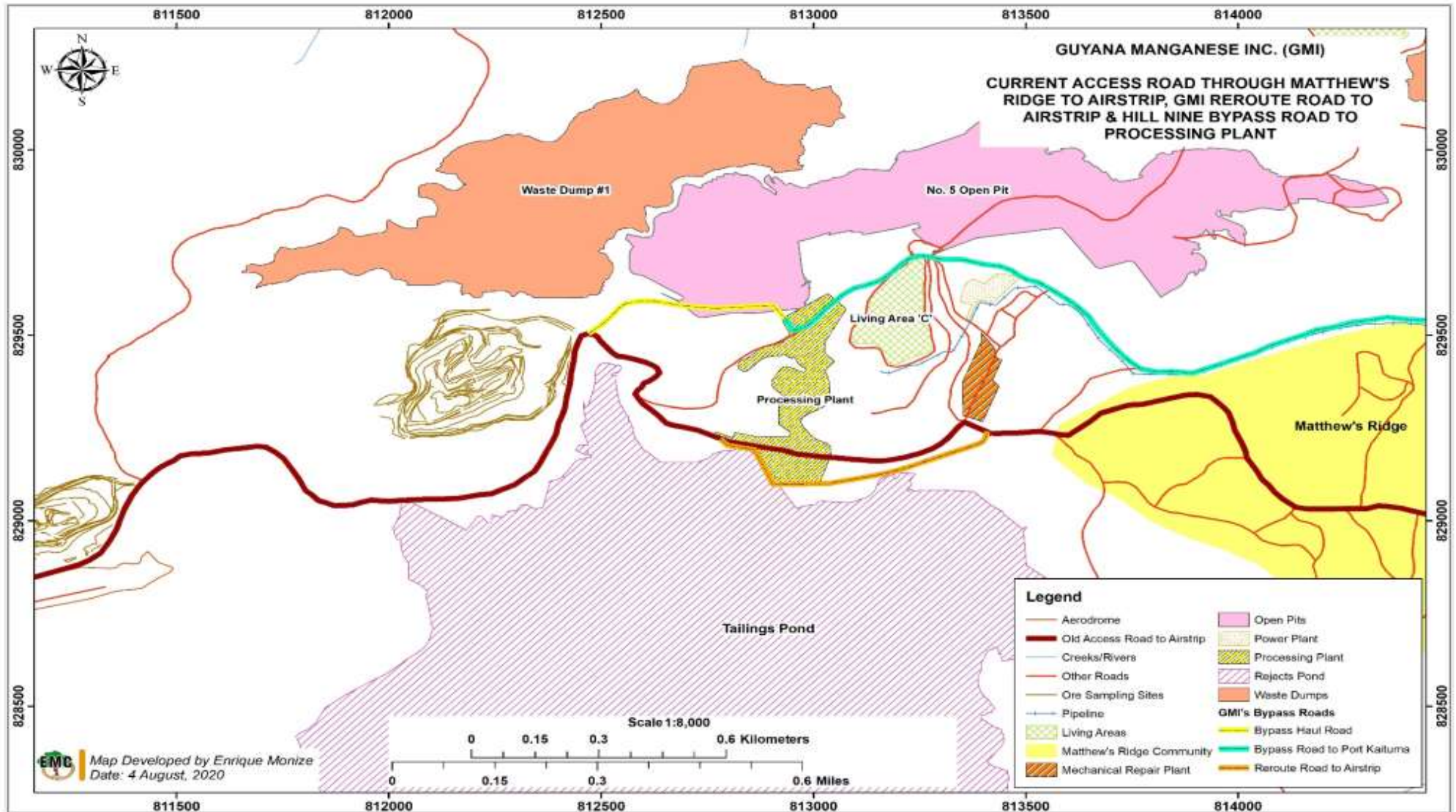
Figure 5-3: Old and Rerouted Access Road to the Airport and Bypass Road to Processing Plant from Hill 9
