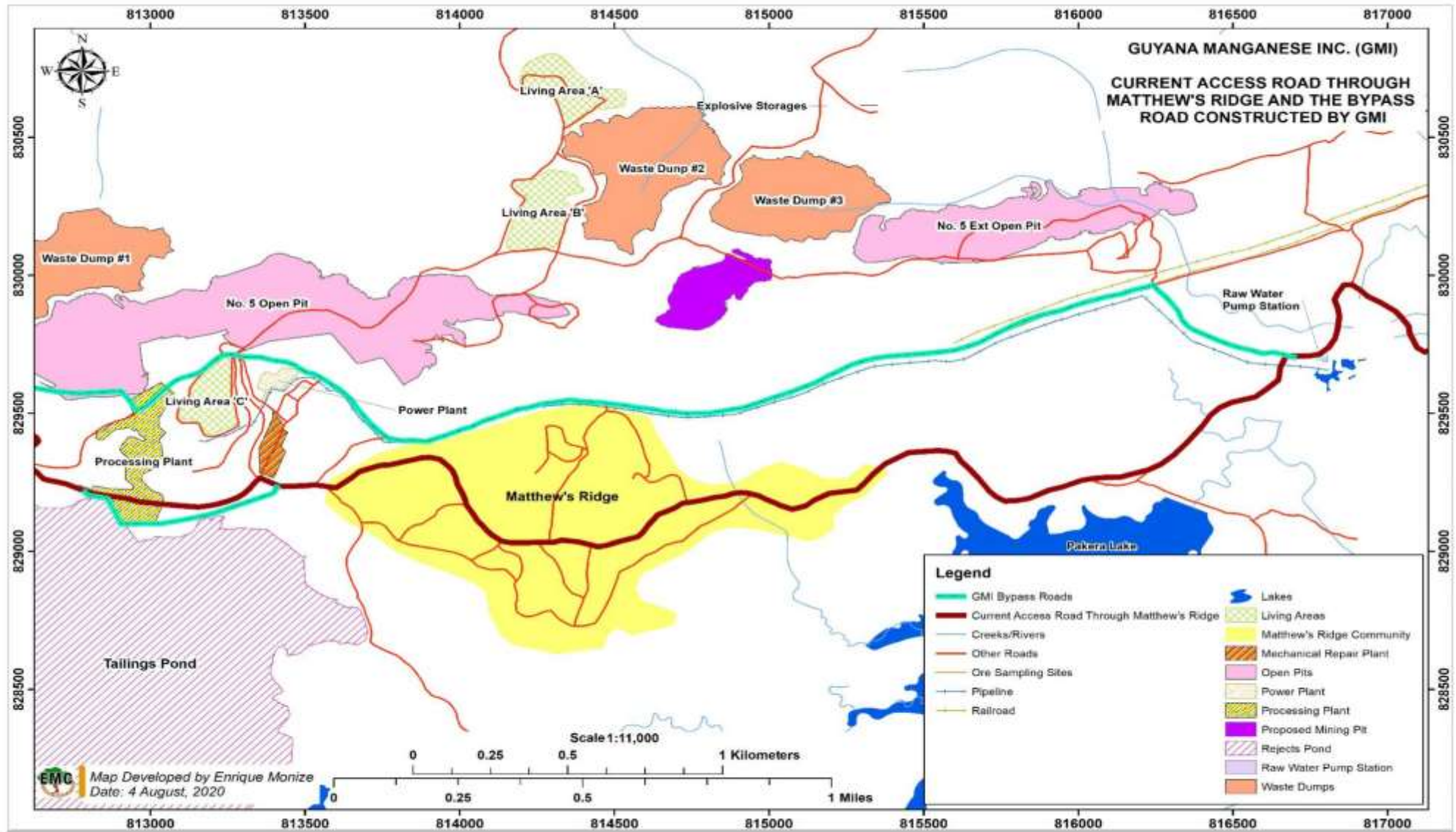
Figure 5-1: Public Road through Matthew's Ridge and Bypass Road Constructed by GMI
