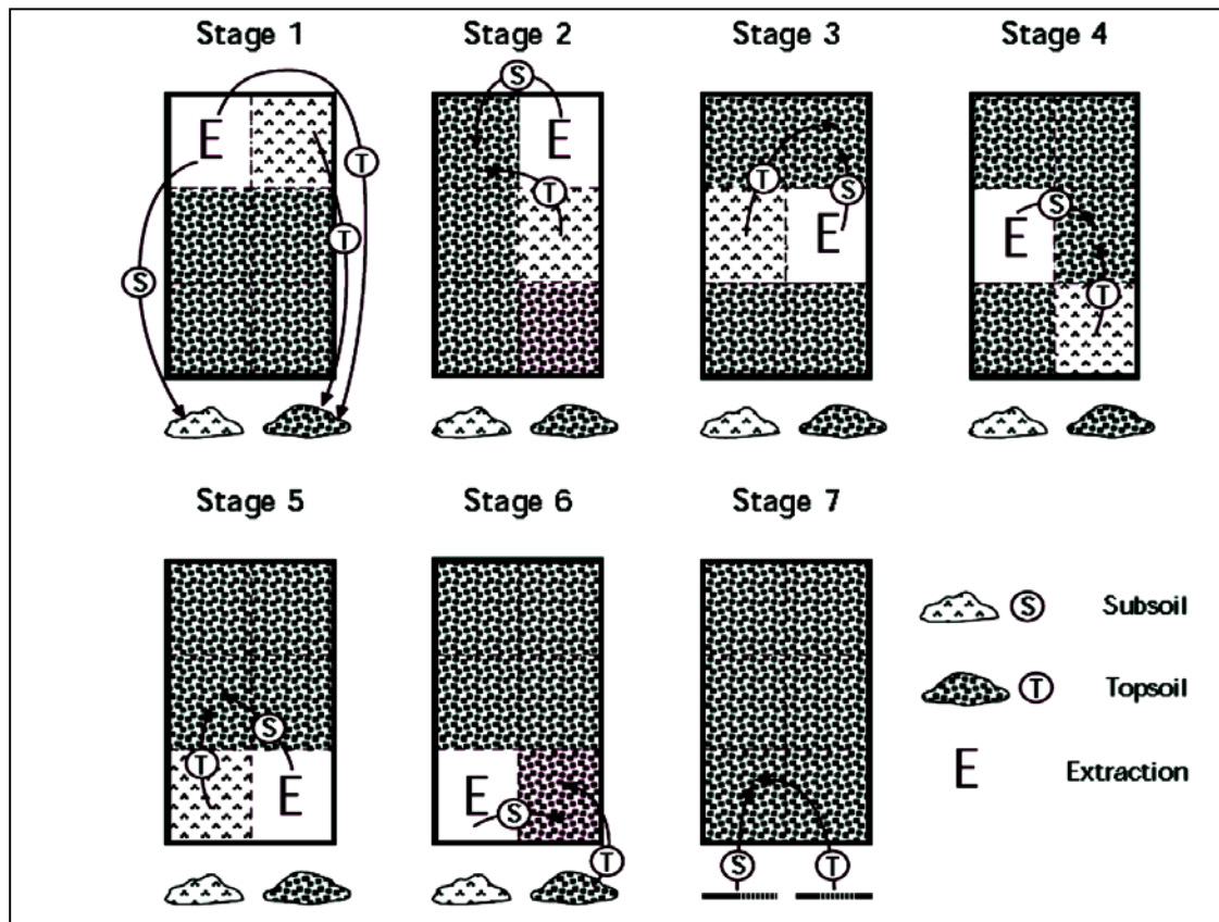
PROGRESSIVE RESTORATION SCHEMATIC PLAN FOR REPLACEMENT OF SOIL
